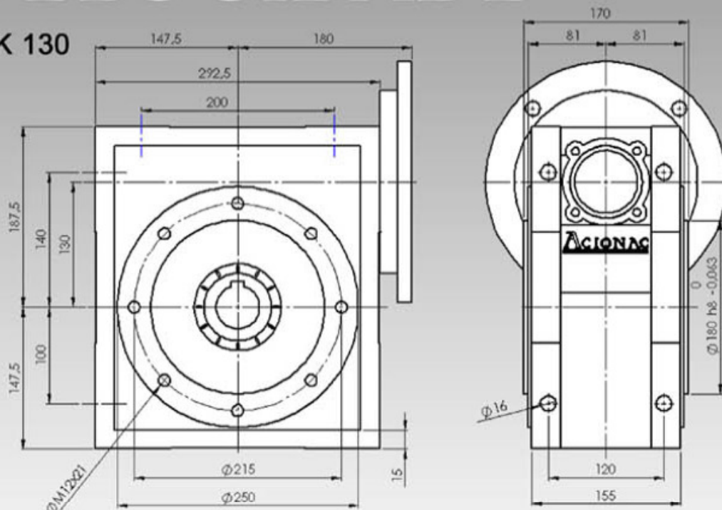
FCNK 130
