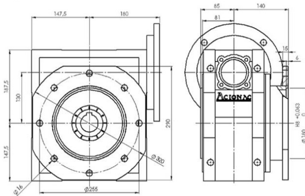
FCNDKO 130 F
