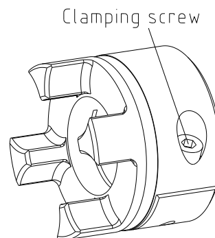
Illustration 20: Assembly of clamping hub
