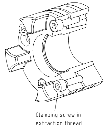
Illustration 22: Disassembly of clamping ring hub with clamping ring
