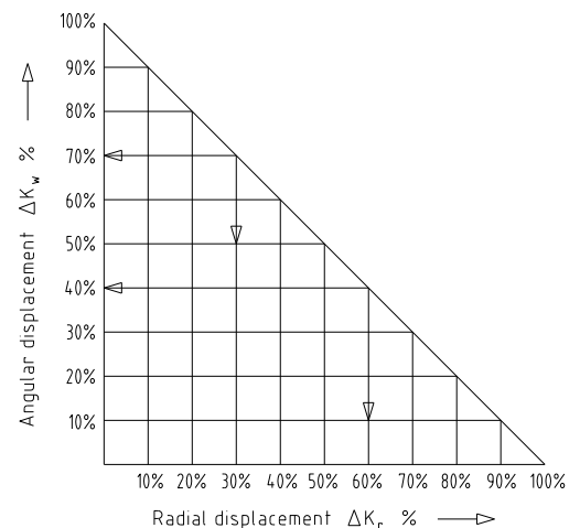
Illustration 24: Combinations of displacement
