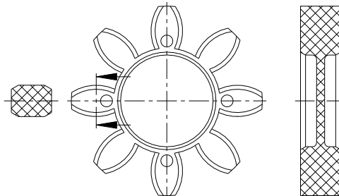
Illustration 26: ROTEX® GS spider
